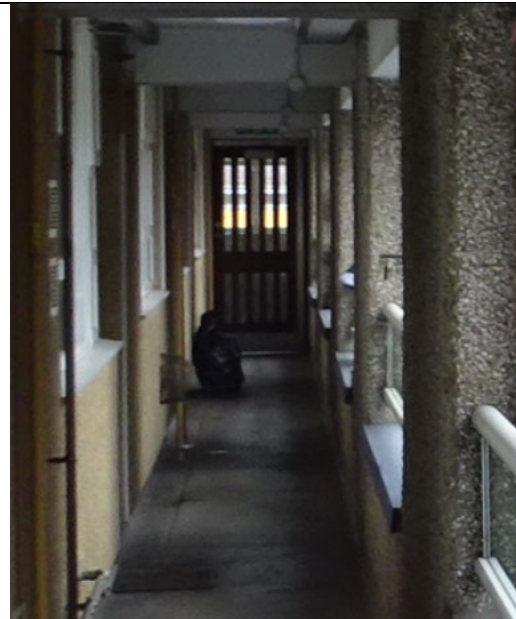
Figure 56: General view to show Fire Door installed at the opposite end of the open access balcony prior to entering the escape staircase and the concrete soffit to the open access balcony.
