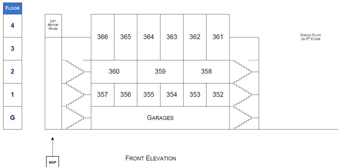
Figure 13: Harold Court West Elevation.
