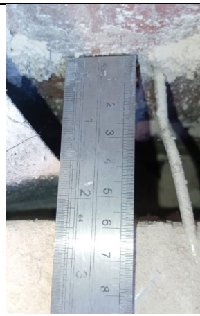
Figure 108: General view to confirm thickness of clear cavity – 60mm.
